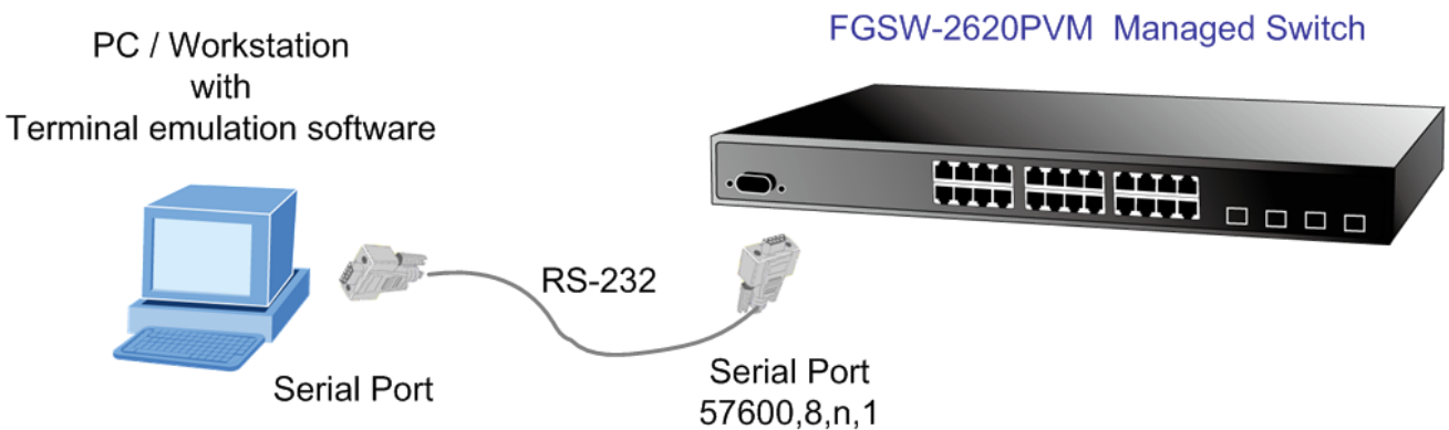
Figure 3-4: Console management
